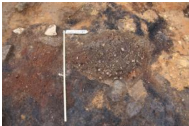
Mynd 9. Hugsanlegar ofnleifar [15] í NV-hluta A5. Fig. 9. Possible furnace remains [15] in NW part of A5.
